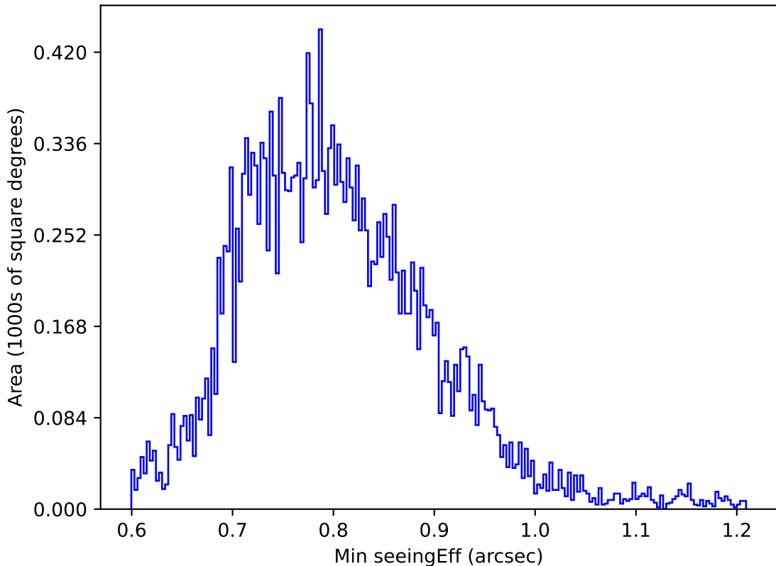
ddf_acor_sf10_lsf15_lsr10_v3.4_10yrs All sky u band: Min seeingEff
