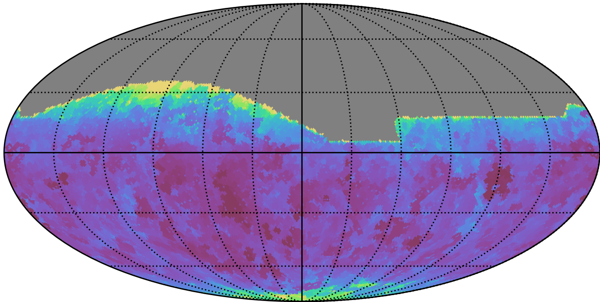
ddf_acor_sf10_lsf15_lsr10_v3.4_10yrs All sky r band: Min seeingEff
