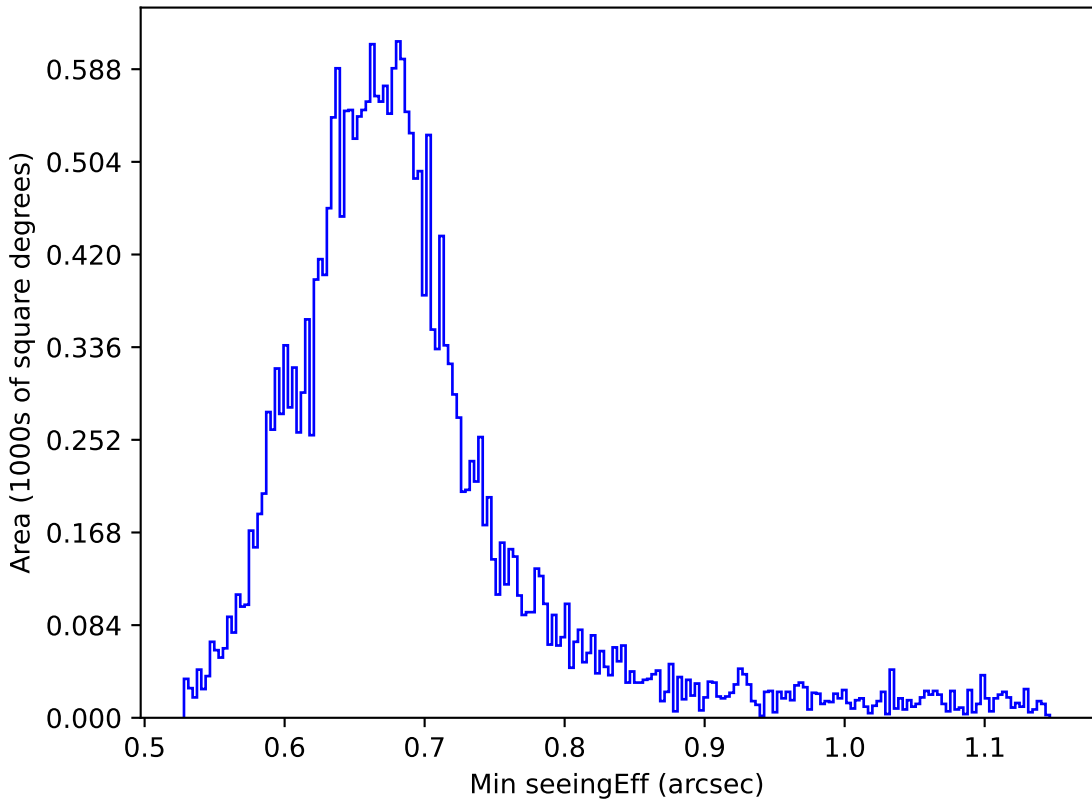
ddf_acor_sf10_lsf15_lsr10_v3.4_10yrs All sky g band: Min seeingEff
