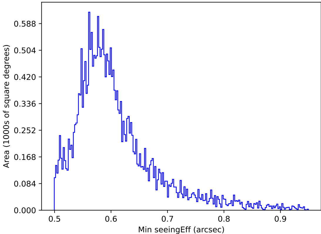
ddf_acor_sf10_lsf15_lsr10_v3.4_10yrs All sky all bands: Min seeingEff
