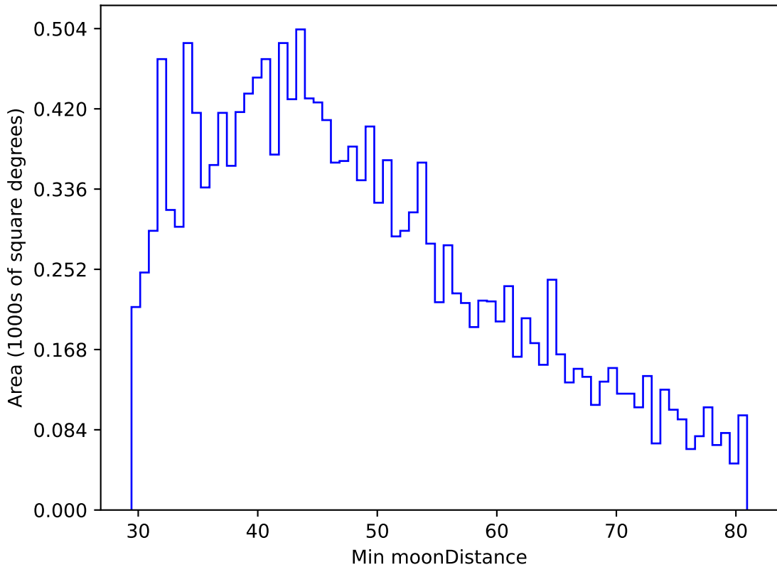
ddf_acor_sf10_lsf15_lsr10_v3.4_10yrs WFD u band: Min moonDistance
