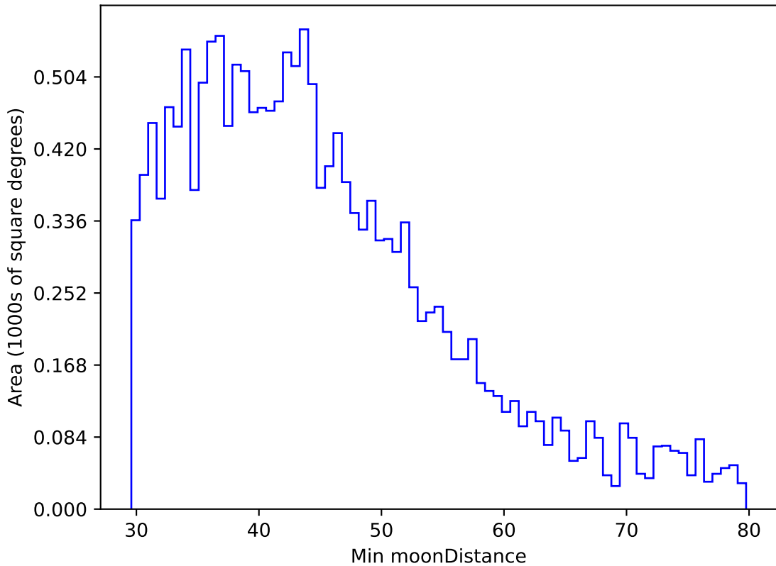
ddf_acor_sf10_lsf15_lsr10_v3.4_10yrs WFD g band: Min moonDistance
