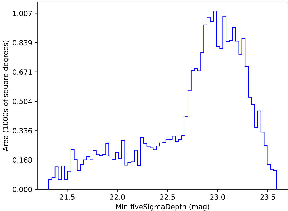
ddf_acor_sf10_lsf15_lsr10_v3.4_10yrs Yr 1 i band: Min fiveSigmaDepth
