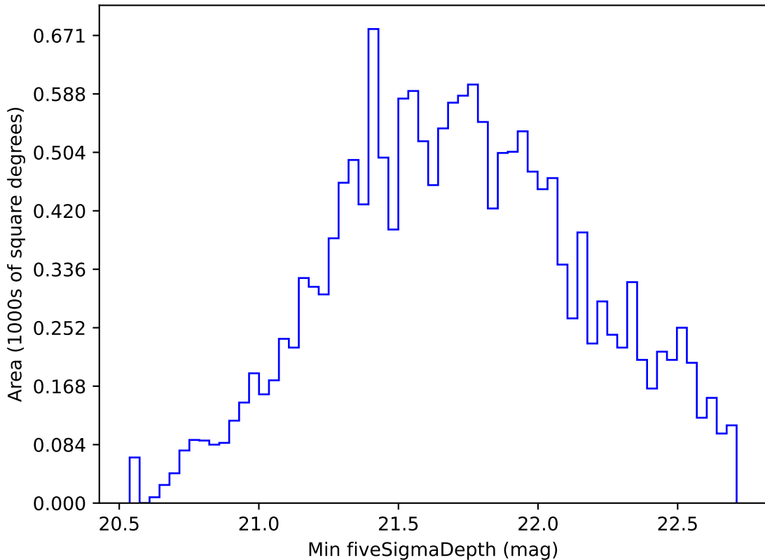
ddf_acor_sf10_lsf15_lsr10_v3.4_10yrs WFD i band: Min fiveSigmaDepth
