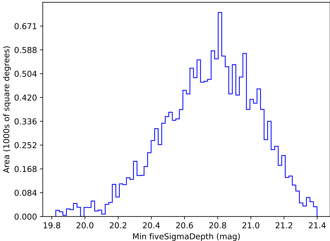
ddf_acor_sf10_ls15_lsr10_v3.4_10yrs WFD all bands: Min fiveSigmaDepth
