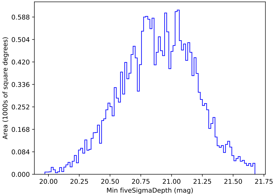
ddf_acor_sf10_lsf15_lsr10_v3.4_10yrs All sky y band: Min fiveSigmaDepth
