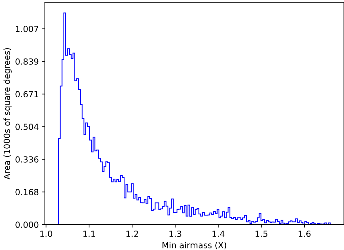
ddf_acor_sf10_lsf15_lsr10_v3.4_10yrs Yr 1 u band: Min airmass
