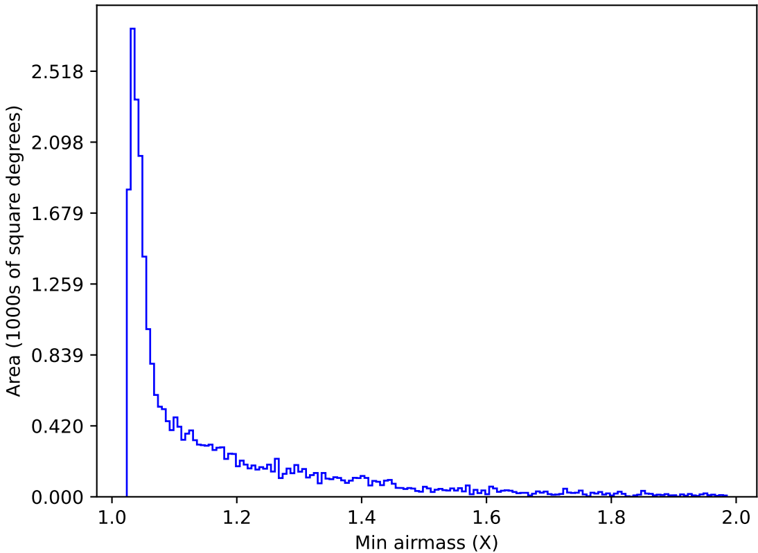
ddf_acor_sf10_lsf15_lsr10_v3.4_10yrs Yr 1 i band: Min airmass
