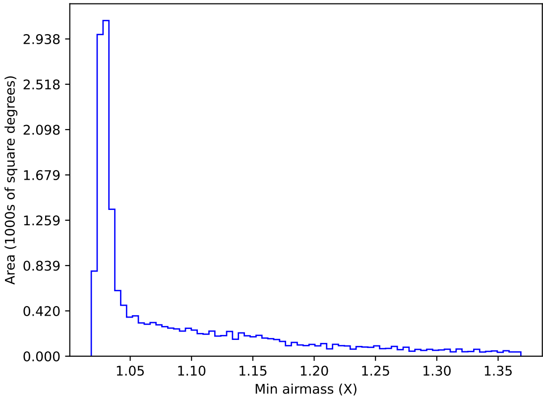
ddf_acor_sf10_lsf15_lsr10_v3.4_10yrs WFD z band: Min airmass
