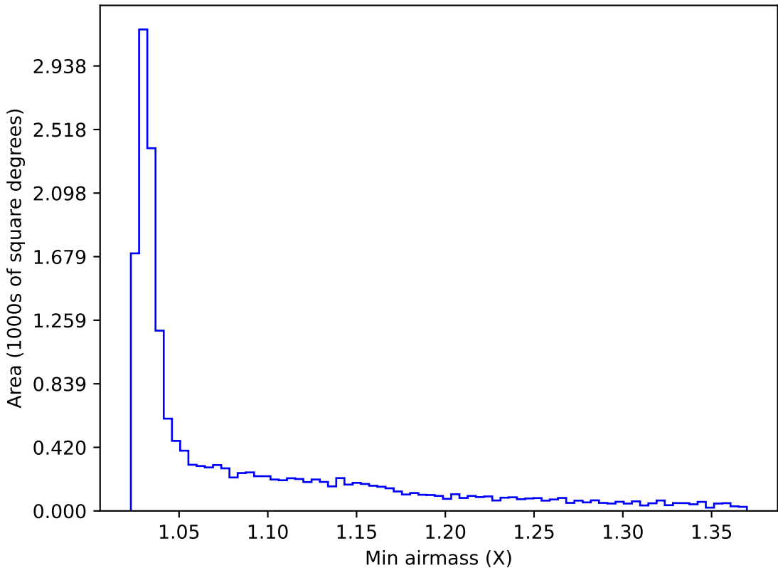
ddf_acor_sf10_lsf15_lsr10_v3.4_10yrs WFD y band: Min airmass
