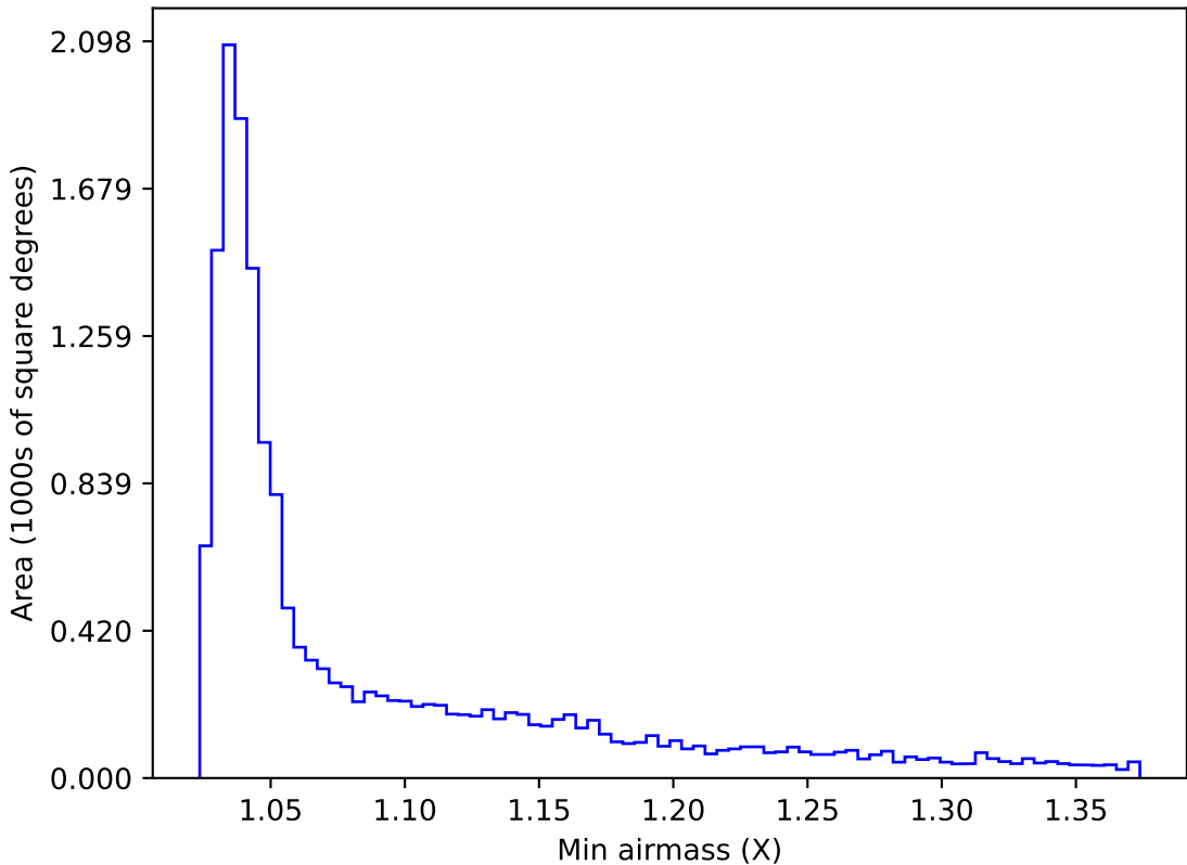
ddf_acor_sf10_lsf15_lsr10_v3.4_10yrs WFD u band: Min airmass
