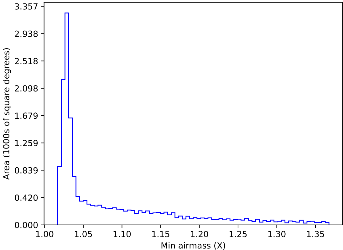
ddf_acor_sf10_lsf15_lsr10_v3.4_10yrs WFD r band: Min airmass
