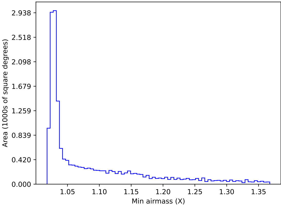
ddf_acor_sf10_lsf15_lsr10_v3.4_10yrs WFD i band: Min airmass
