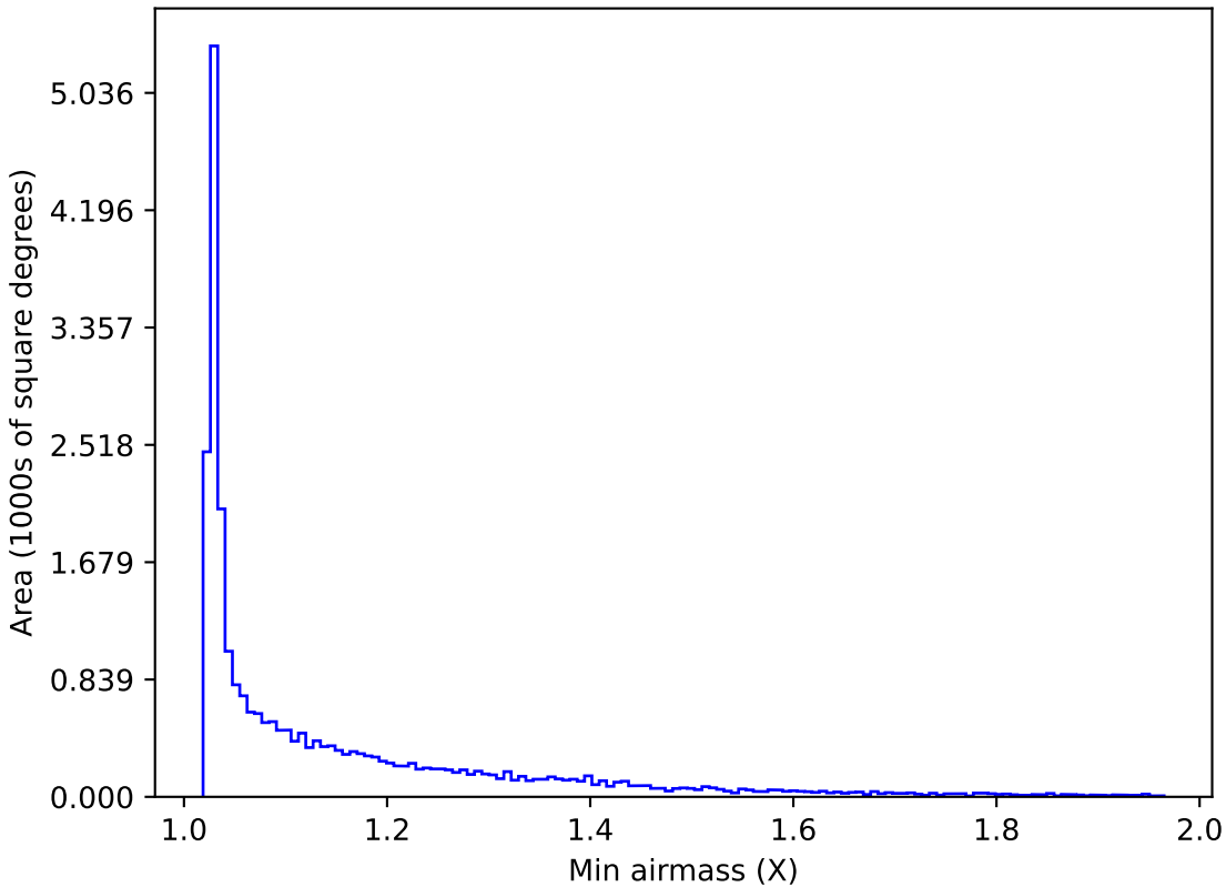
ddf_acor_sf10_lsf15_lsr10_v3.4_10yrs All sky z band: Min airmass
