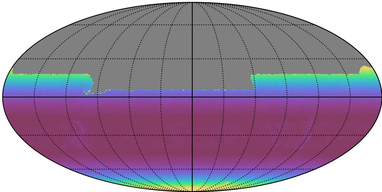
ddf_acor_sf10_lsf15_lsr10_v3.4_10yrs All sky y band: Min airmass
