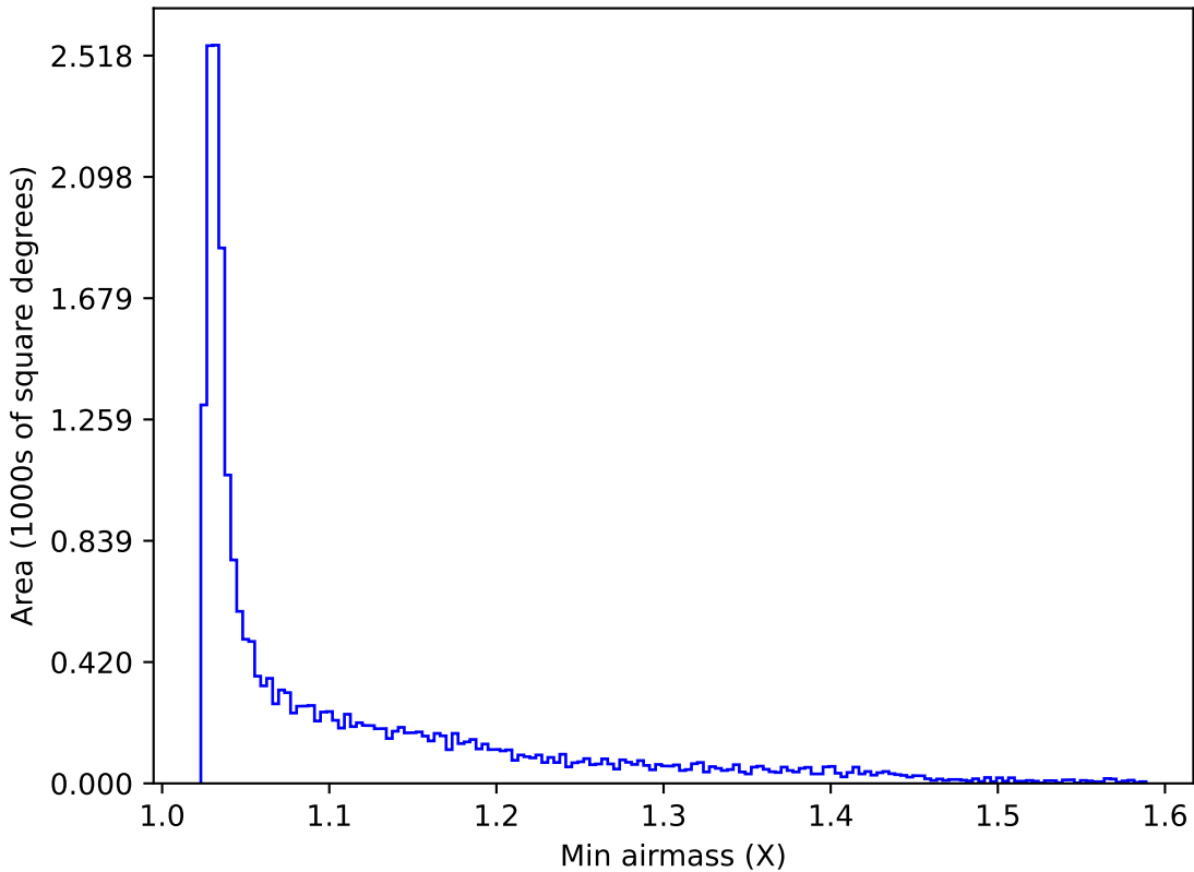
ddf_acor_sf10_lsf15_lsr10_v3.4_10yrs All sky y band: Min airmass
