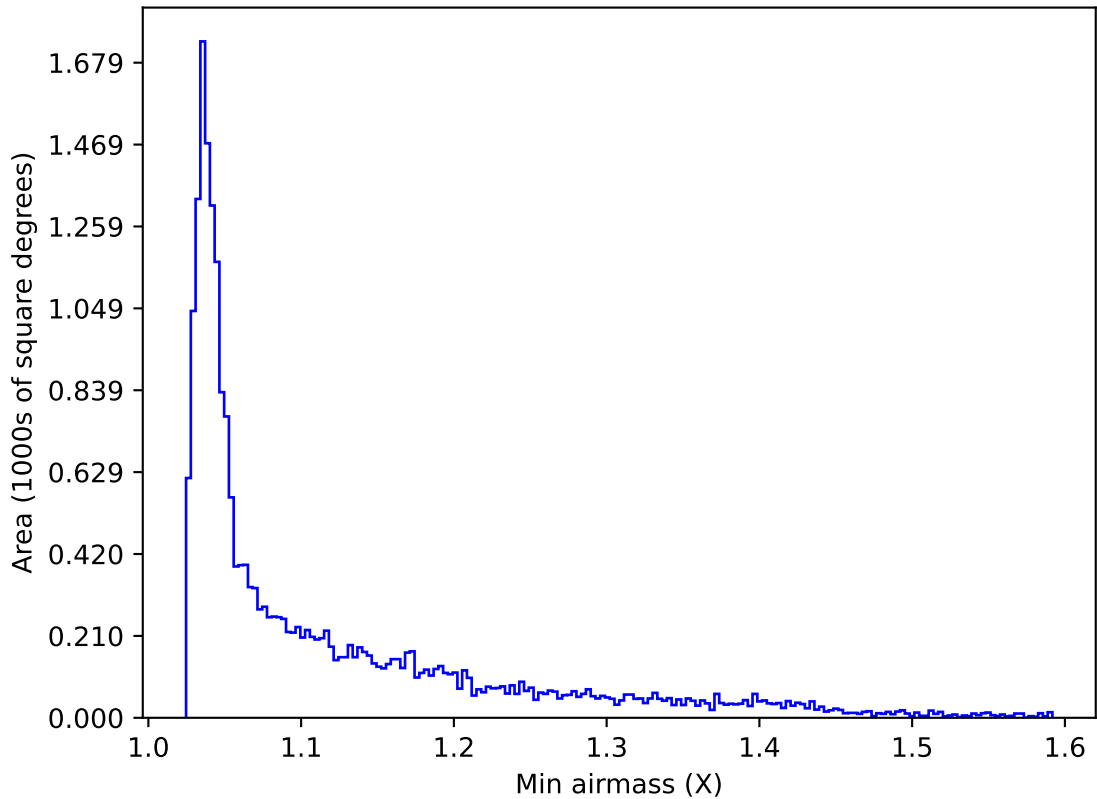
ddf_acor_sf10_lsf15_lsr10_v3.4_10yrs All sky u band: Min airmass
