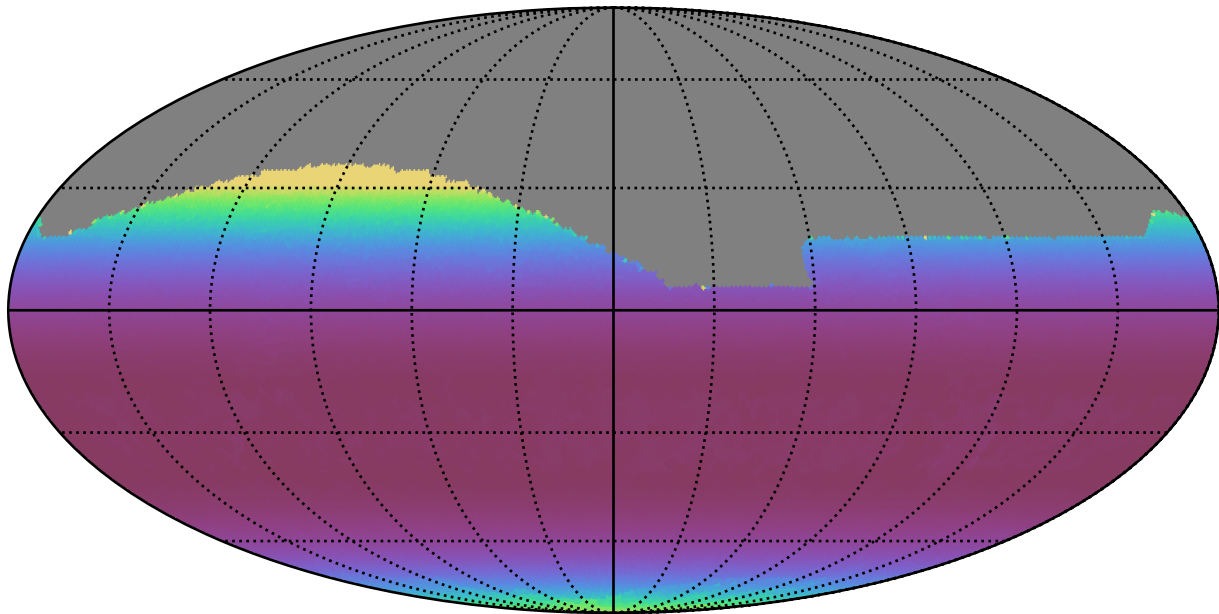
ddf_acor_sf10_lsf15_lsr10_v3.4_10yrs All sky r band: Min airmass
