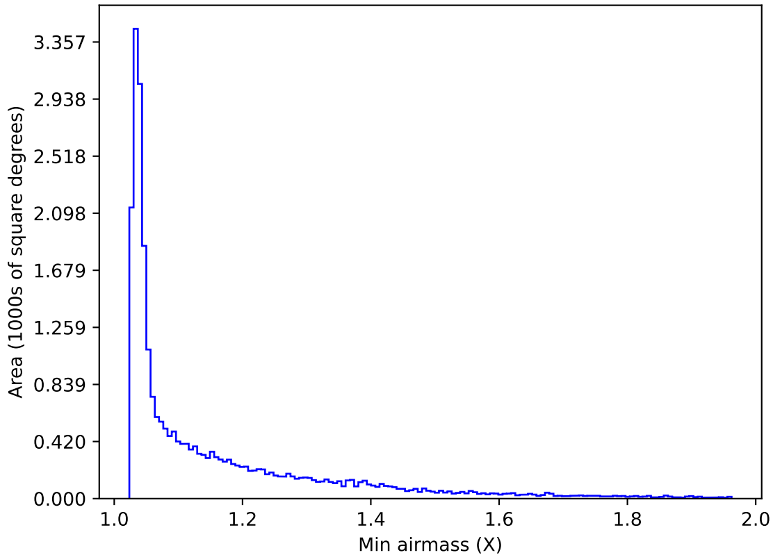
ddf_acor_sf10_lsf15_lsr10_v3.4_10yrs All sky g band: Min airmass
