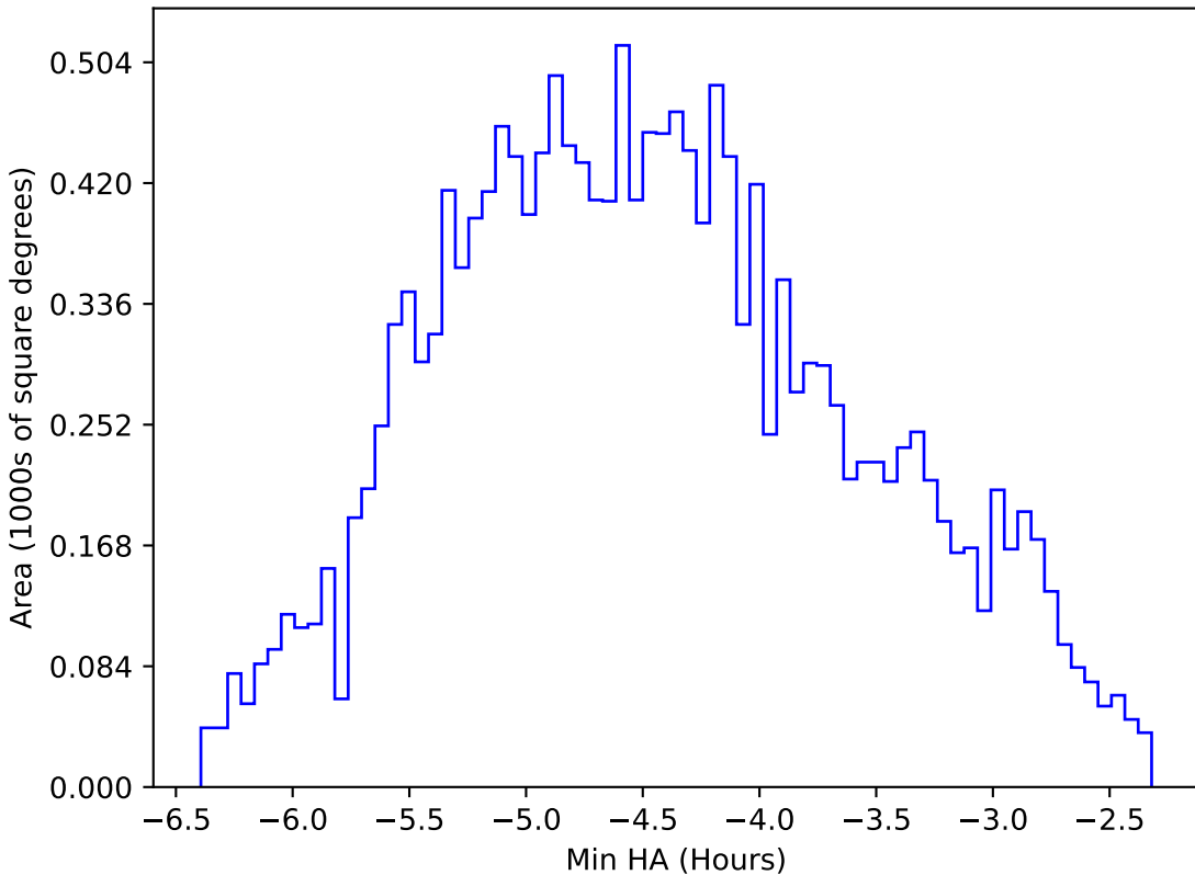
ddf_acor_sf10_lsf15_lsr10_v3.4_10yrs WFD r band: Min HA
