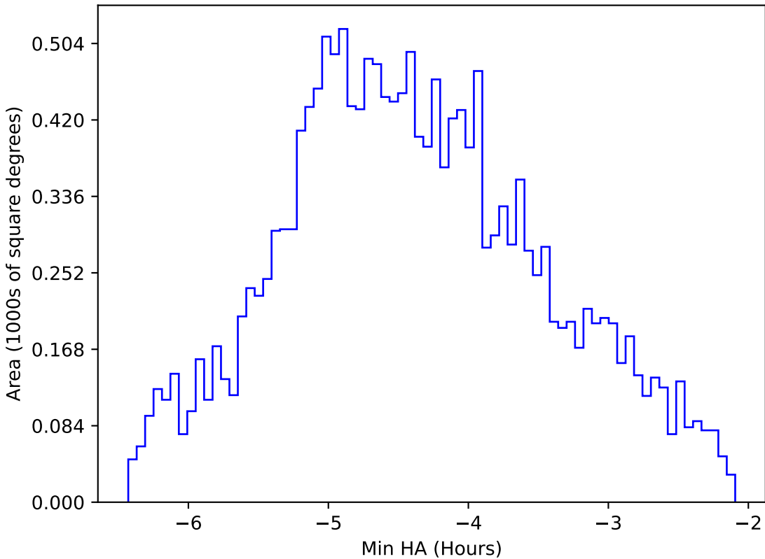
ddf_acor_sf10_lsf15_lsr10_v3.4_10yrs WFD i band: Min HA
