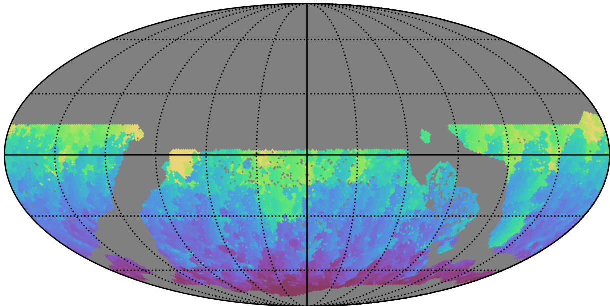
ddf_acor_sf10_lsf15_lsr10_v3.4_10yrs WFD g band: Min HA
