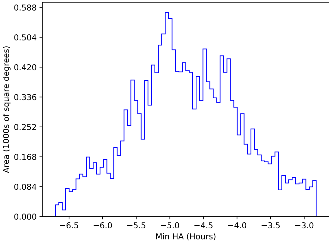
ddf_acor_sf10_ls15_lsr10_v3.4_10yrs WFD all bands: Min HA
