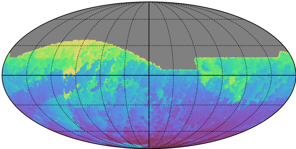
ddf_acor_sf10_lsf15_lsr10_v3.4_10yrs All sky z band: Min HA
