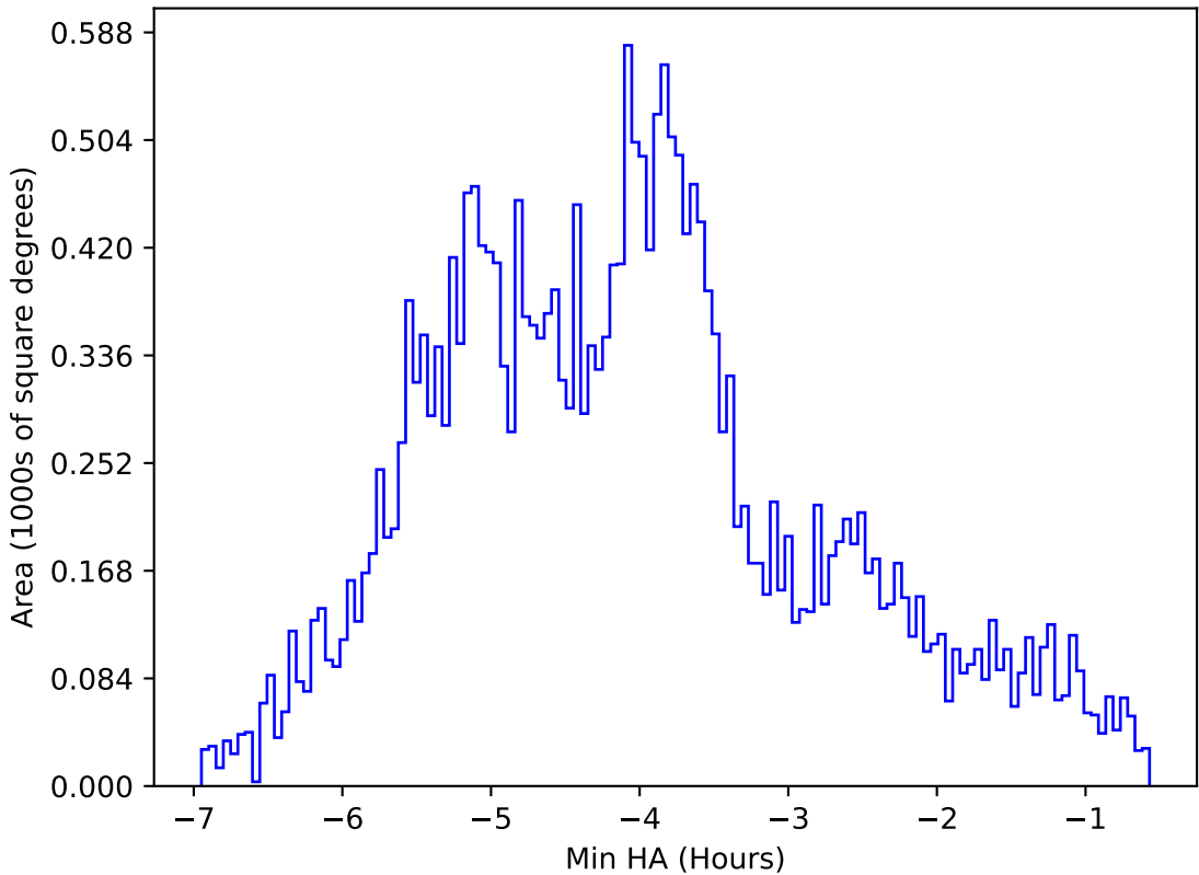
ddf_acor_sf10_lsf15_lsr10_v3.4_10yrs All sky z band: Min HA
