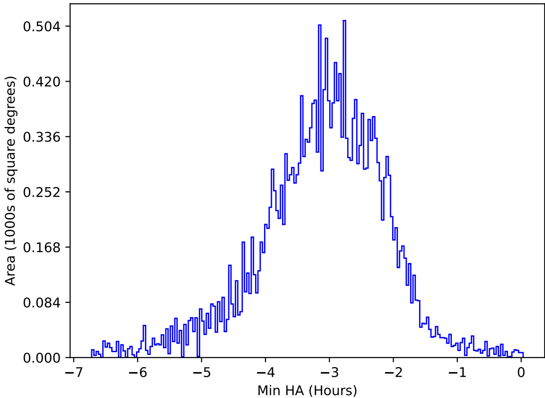
ddf_acor_sf10_ls15_lsr10_v3.4_10yrs All sky u band: Min HA
