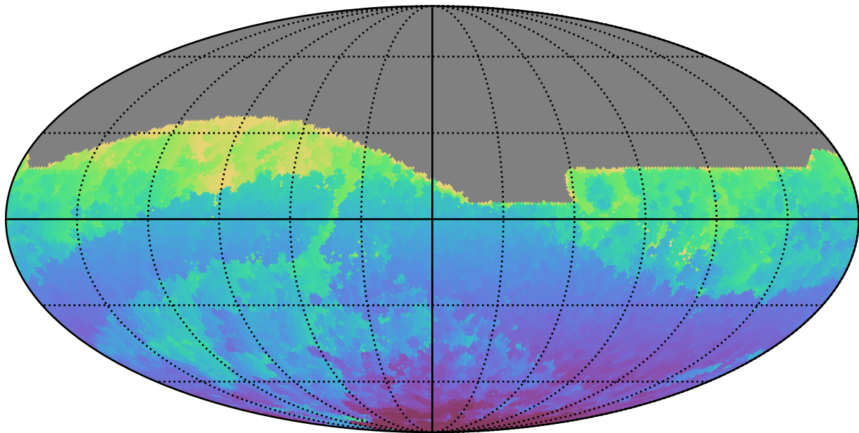
ddf_acor_sf10_lsf15_lsr10_v3.4_10yrs All sky r band: Min HA
