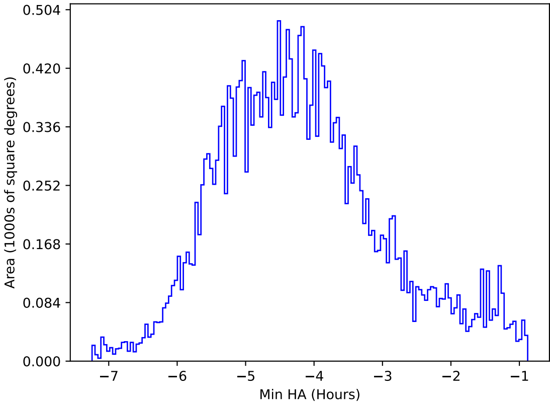
ddf_acor_sf10_ls15_lsr10_v3.4_10yrs All sky r band: Min HA
