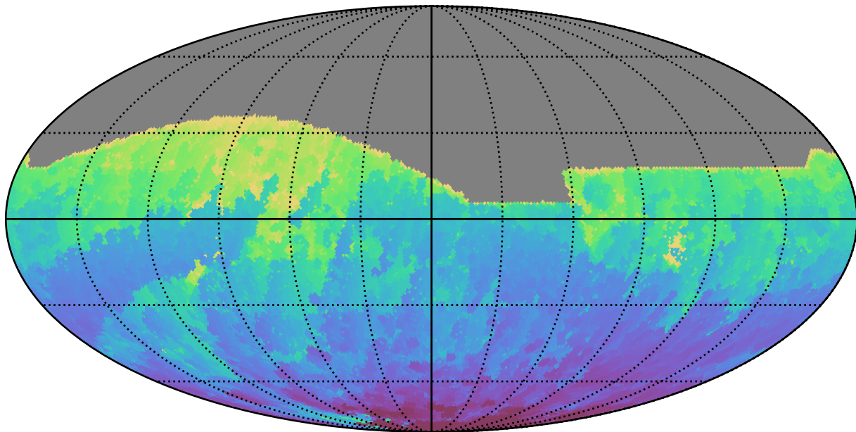
ddf_acor_sf10_lsf15_lsr10_v3.4_10yrs All sky i band: Min HA
