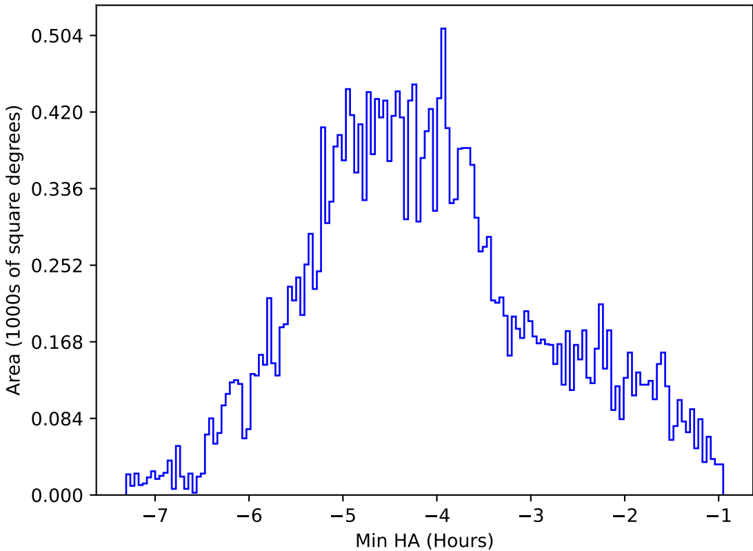
ddf_acor_sf10_ls15_lsr10_v3.4_10yrs All sky i band: Min HA
