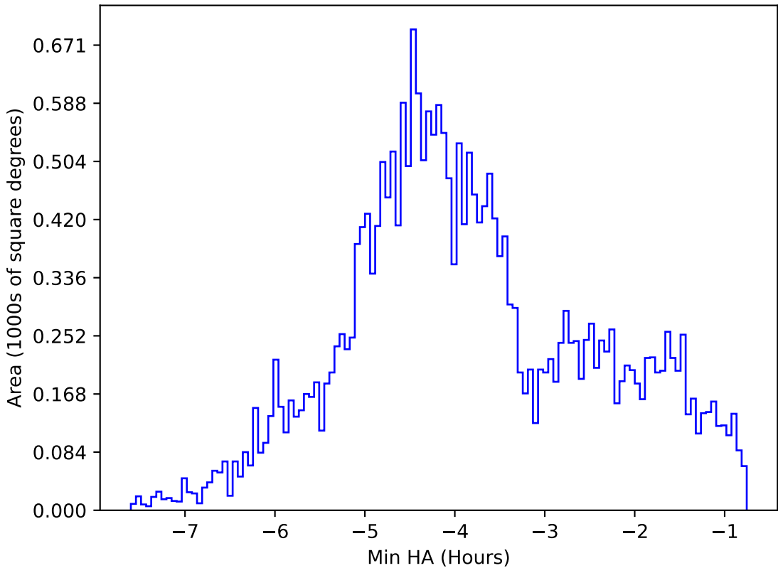
ddf_acor_sf10_ls15_lsr10_v3.4_10yrs All sky g band: Min HA
