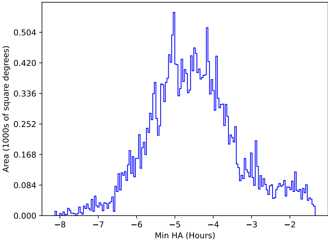
ddf_acor_sf10_lsf15_lsr10_v3.4_10yrs All sky all bands: Min HA
