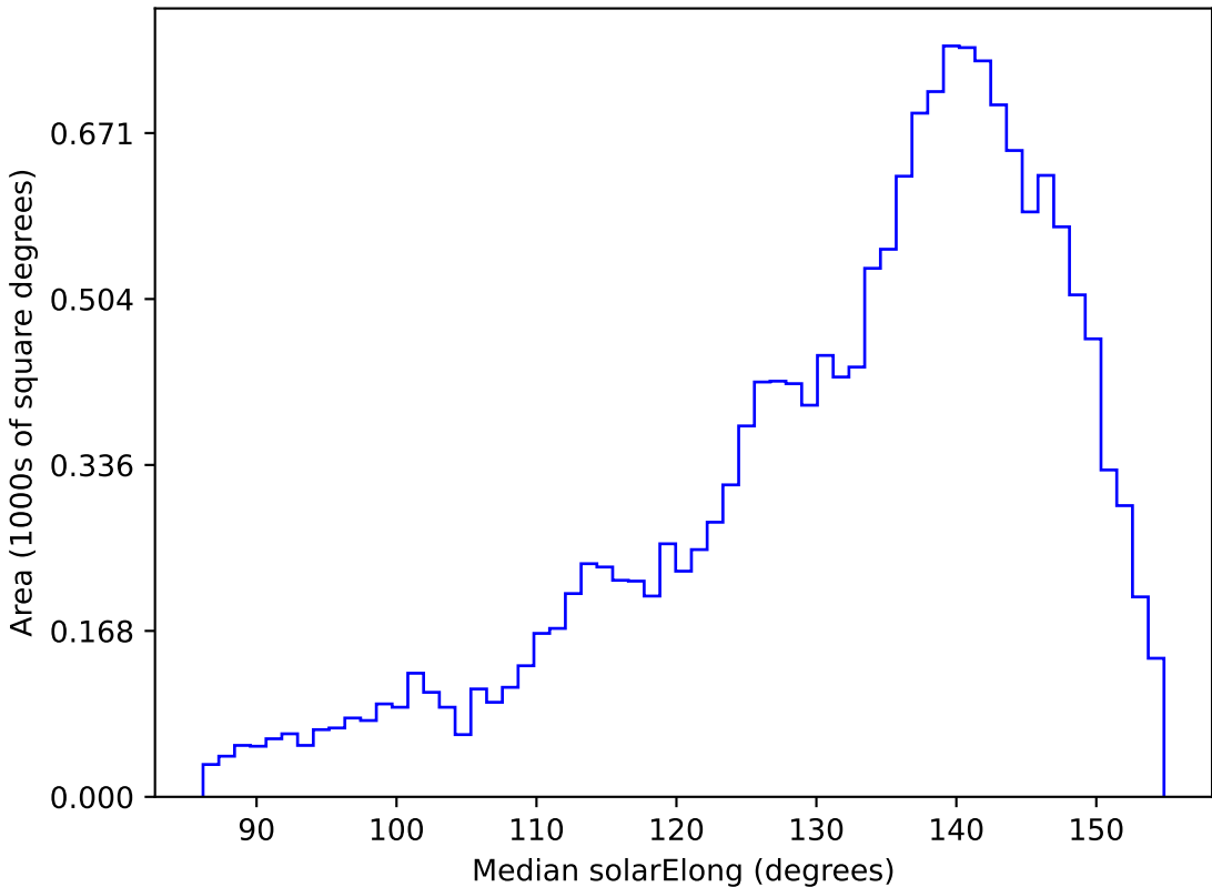
ddf_acor_sf10_lsf15_lsr10_v3.4_10yrs WFD u band: Median solarElong
