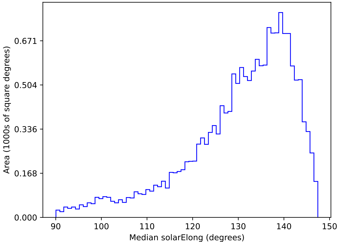
ddf_acor_sf10_lsf15_lsr10_v3.4_10yrs WFD r band: Median solarElong
