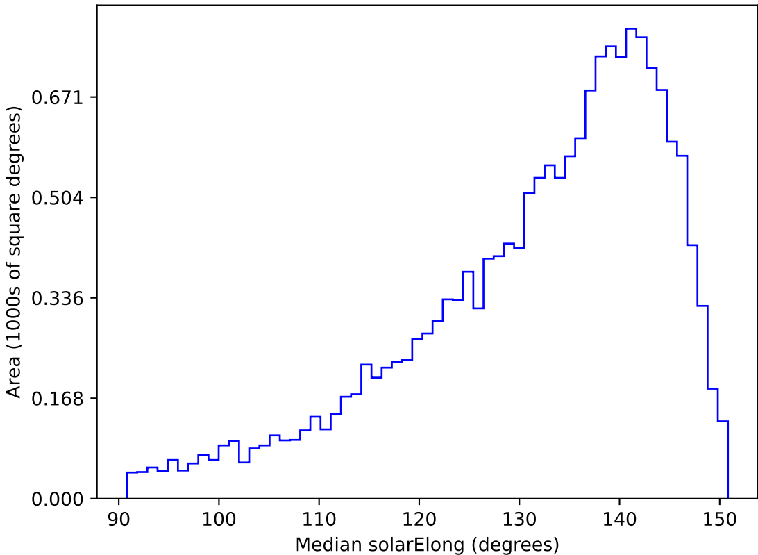
ddf_acor_sf10_lsf15_lsr10_v3.4_10yrs WFD g band: Median solarElong
