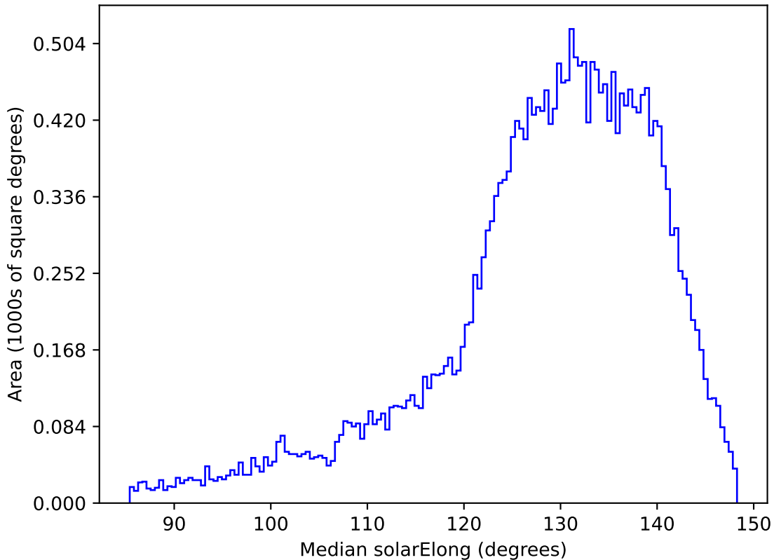
ddf_acor_sf10_lsf15_lsr10_v3.4_10yrs All sky i band: Median solarElong
