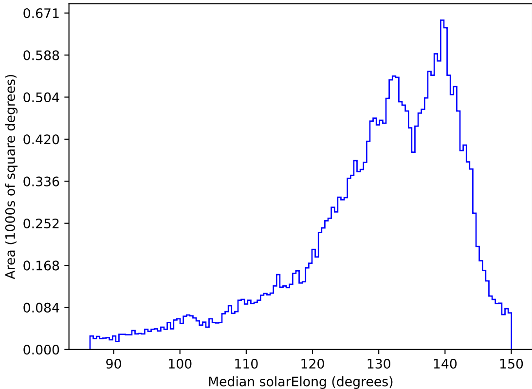
ddf_acor_sf10_lsf15_lsr10_v3.4_10yrs All sky all bands: Median solarElong
