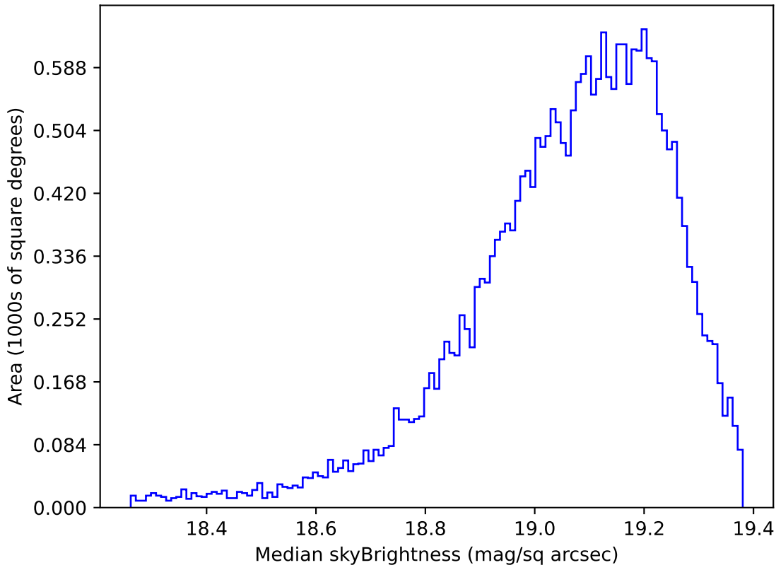
ddf_acor_sf10_lsf15_lsr10_v3.4_10yrs Yr 1 z band: Median skyBrightness
