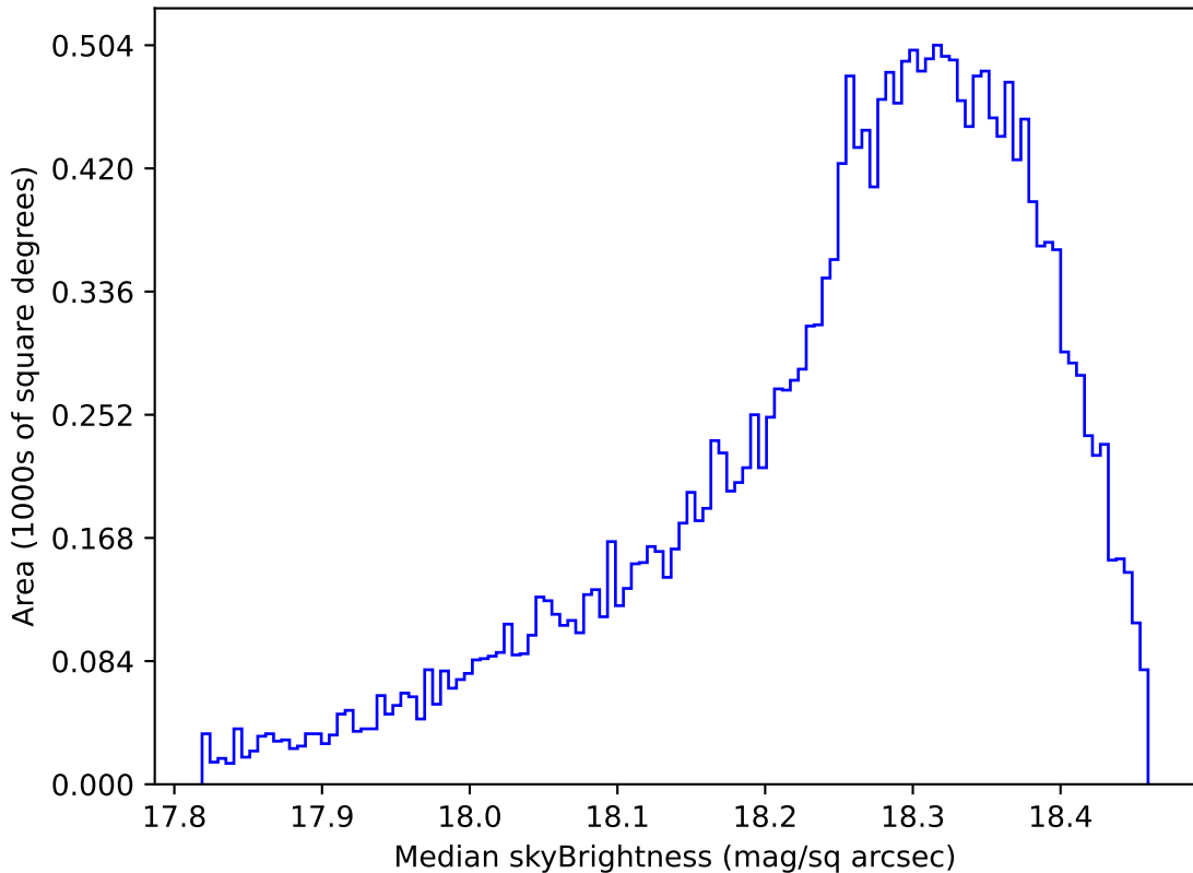
ddf_acor_sf10_lsf15_lsr10_v3.4_10yrs Yr 1 y band: Median skyBrightness
