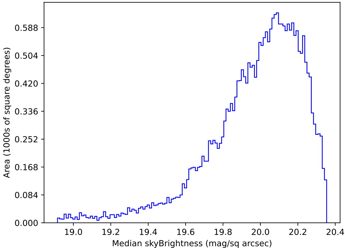
ddf_acor_sf10_lsf15_lsr10_v3.4_10yrs Yr 1 i band: Median skyBrightness
