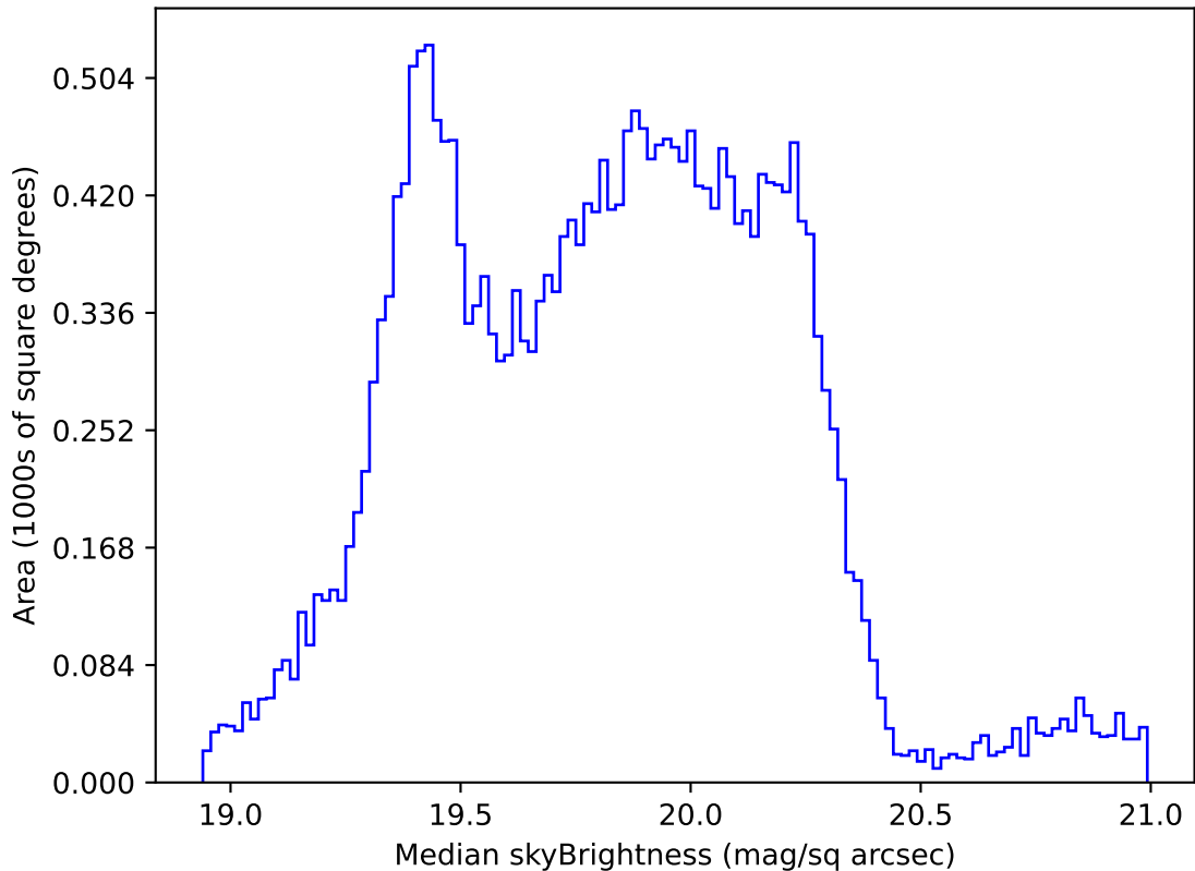
ddf_acor_sf10_lsf15_lsr10_v3.4_10yrs Yr 1 all bands: Median skyBrightness
