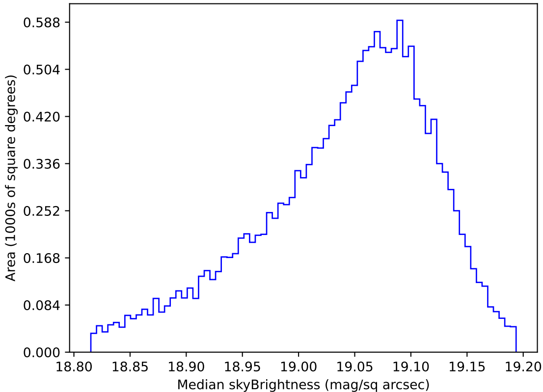
ddf_acor_sf10_lsf15_lsr10_v3.4_10yrs WFD z band: Median skyBrightness
