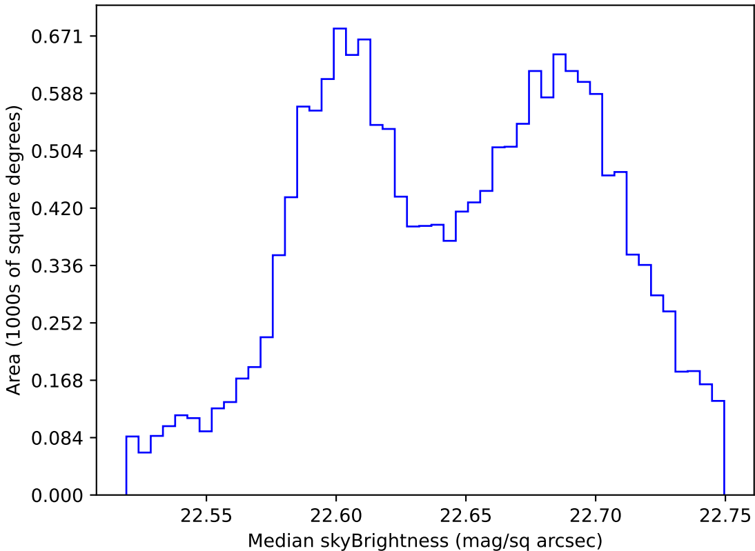
ddf_acor_sf10_lsf15_lsr10_v3.4_10yrs WFD u band: Median skyBrightness
