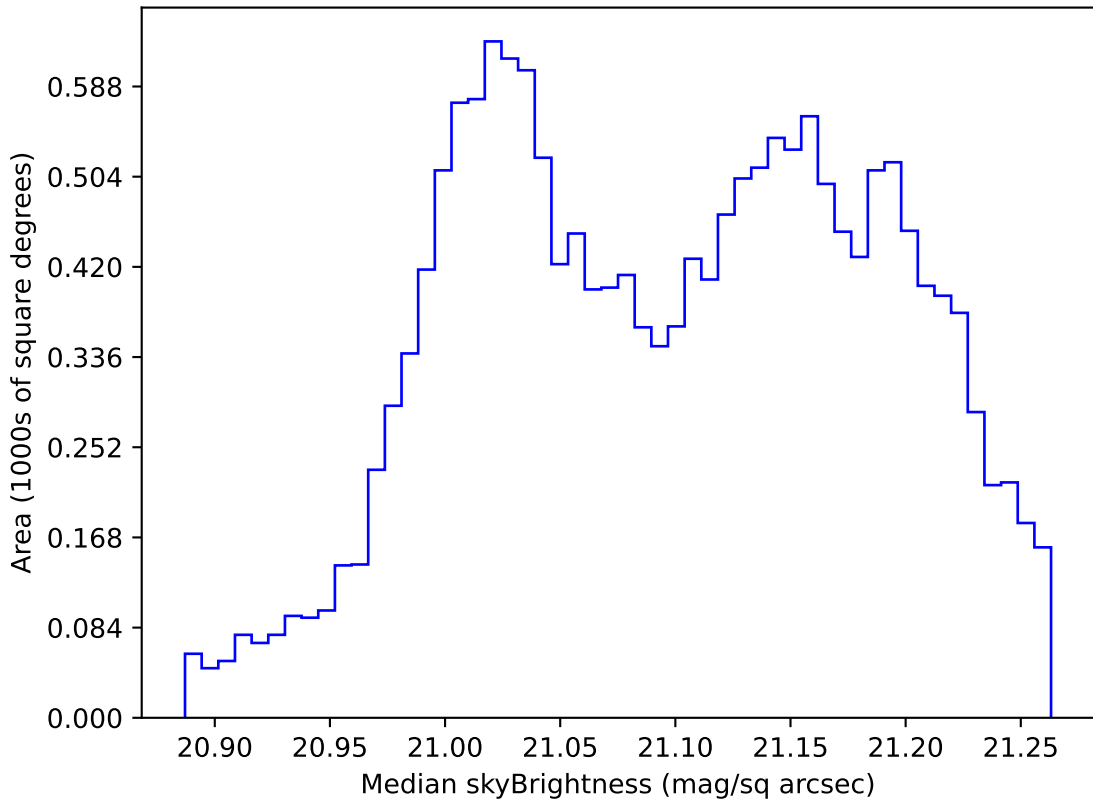
ddf_acor_sf10_lsf15_lsr10_v3.4_10yrs WFD r band: Median skyBrightness
