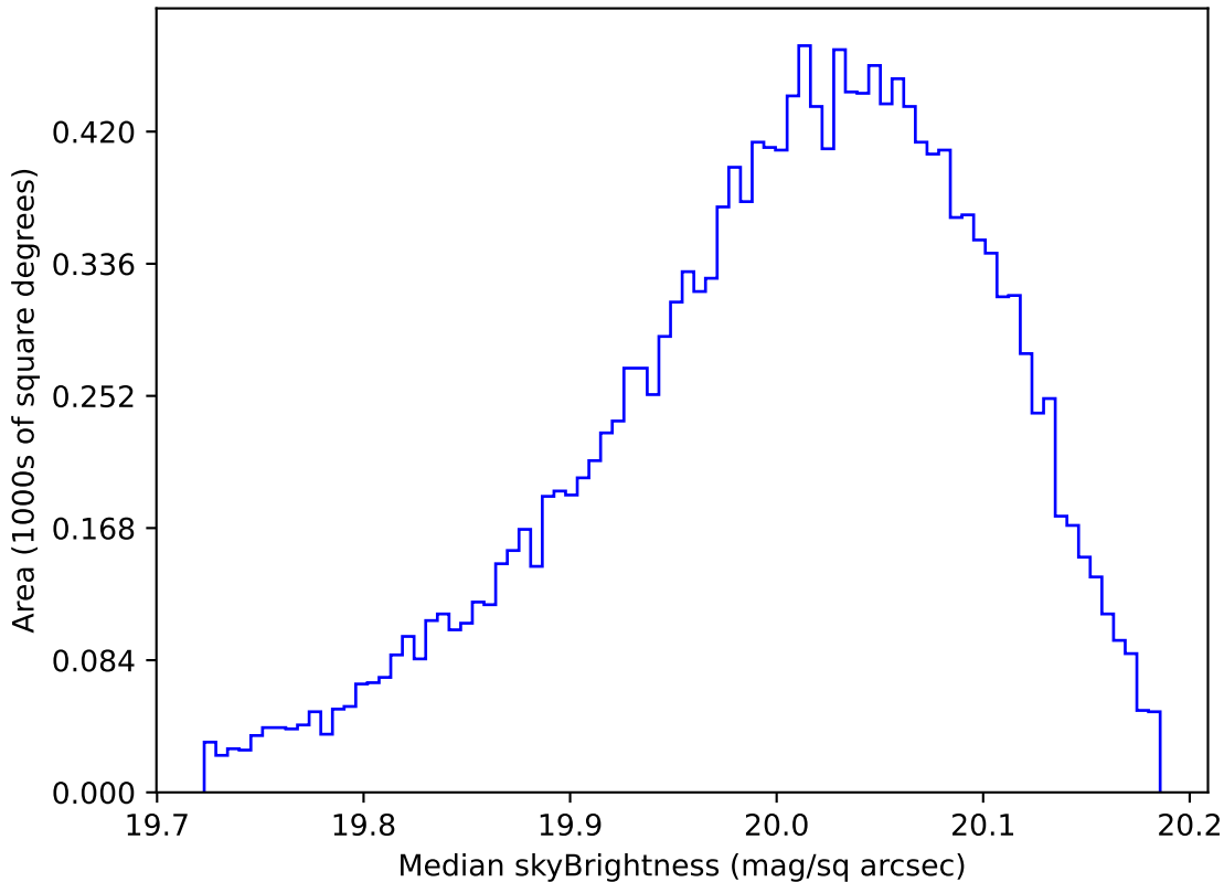
ddf_acor_sf10_lsf15_lsr10_v3.4_10yrs WFD i band: Median skyBrightness
