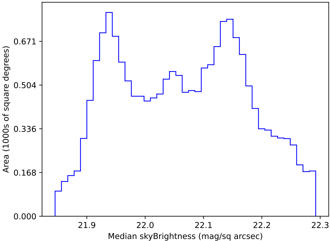
ddf_acor_sf10_lsf15_lsr10_v3.4_10yrs WFD g band: Median skyBrightness
